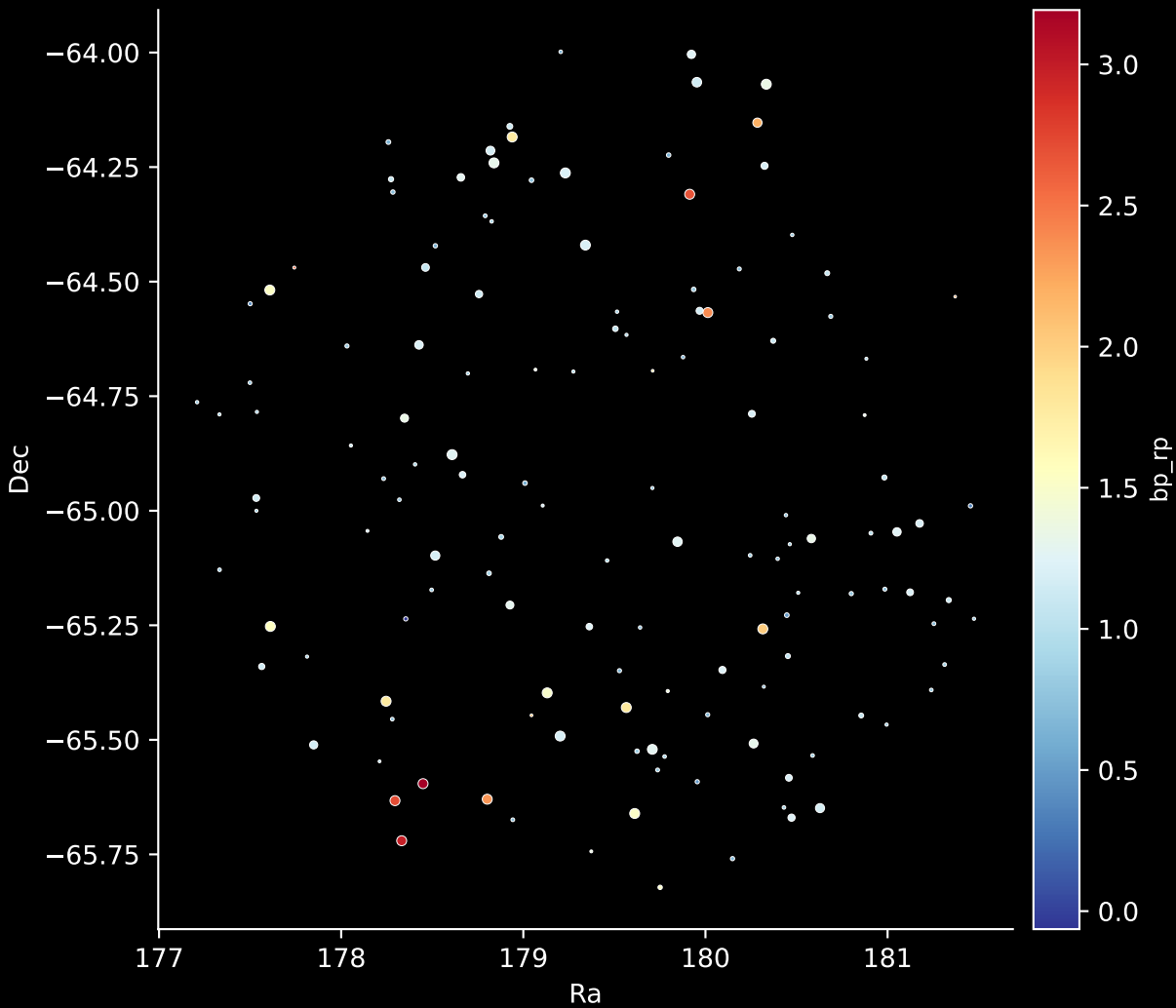
APOGEE DR17 Field: [275-34-O_TESS] Stars: 137
