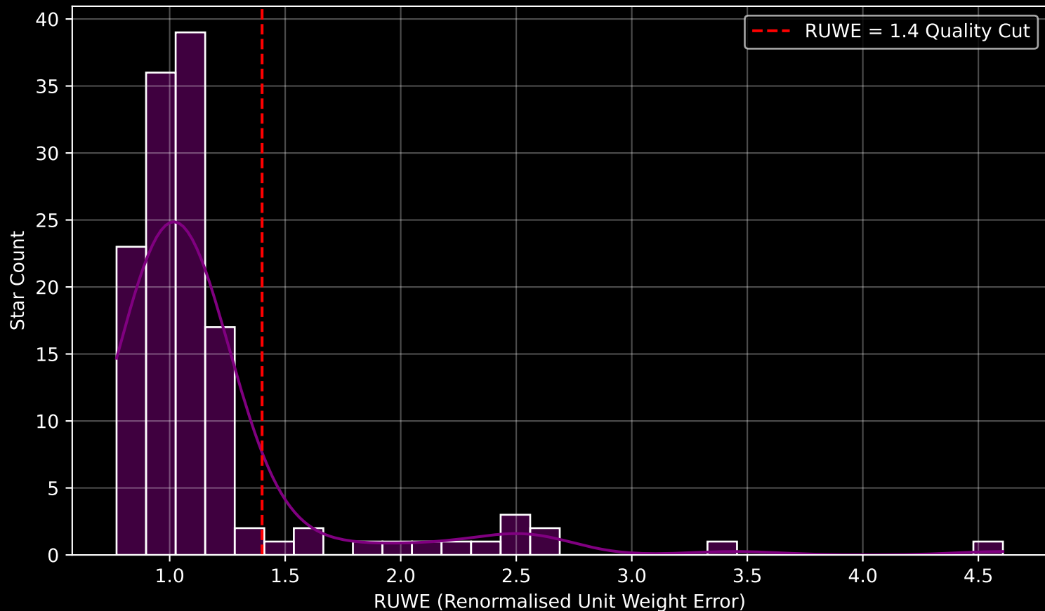
GAPOGEE DR17 Field [275-34-O_TESS] RUWE Distribution (n= 132)
