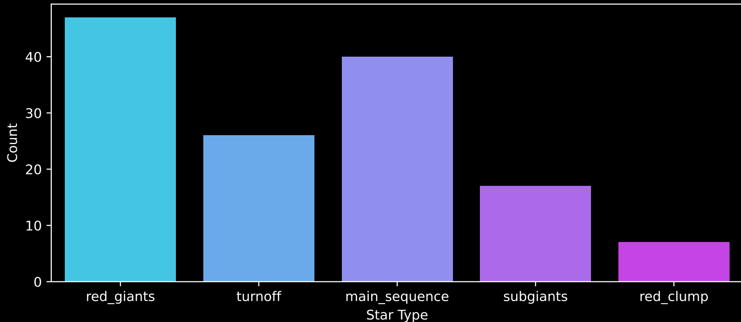
APOGEE DR17 Field: [275-34-O_TESS] Count plot of Star Type
