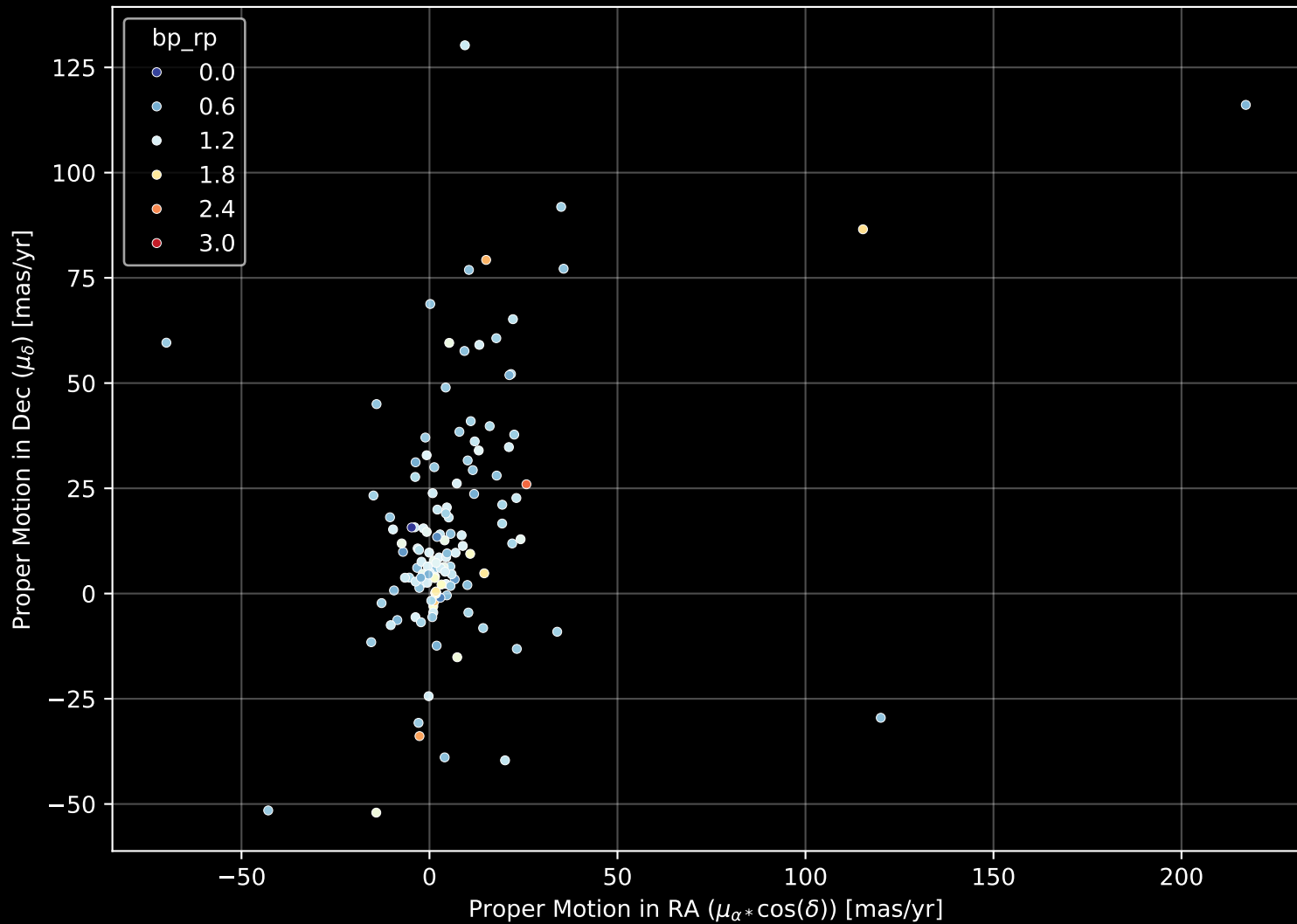
APOGEE DR17 Field: [275-34-O_TESS] Proper Motion Diagram (n= 137)
