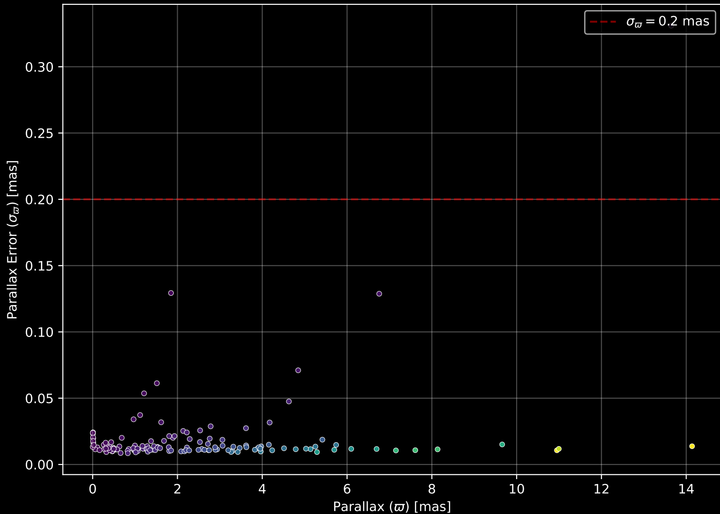
APOGEE DR17 Field: [275-34-O_TESS] Parallax Quality (n= 137)
