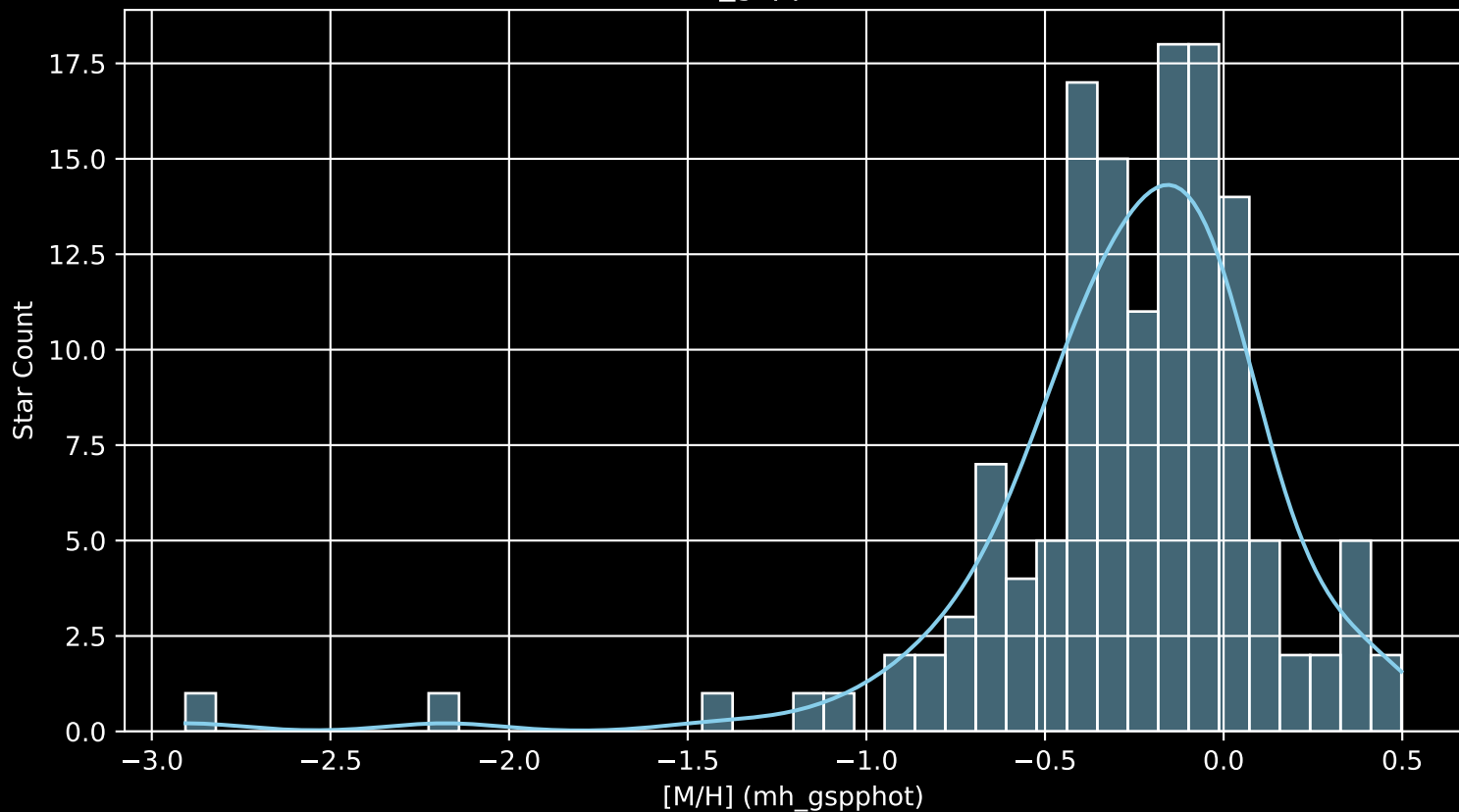
APOGEE DR17 Field: [275-34-O_TESS [M/H] (mh_gspphot) (n= 137)
